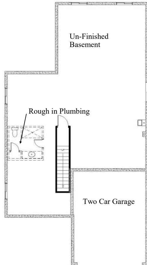
Unfinished Basement Plan
