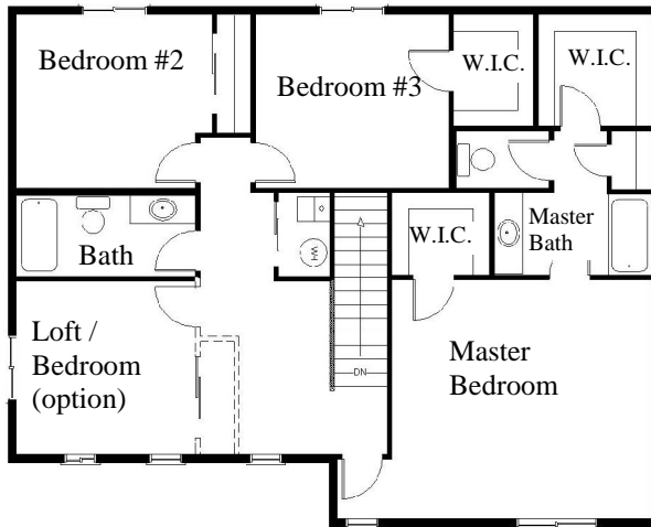
Upper Floor
