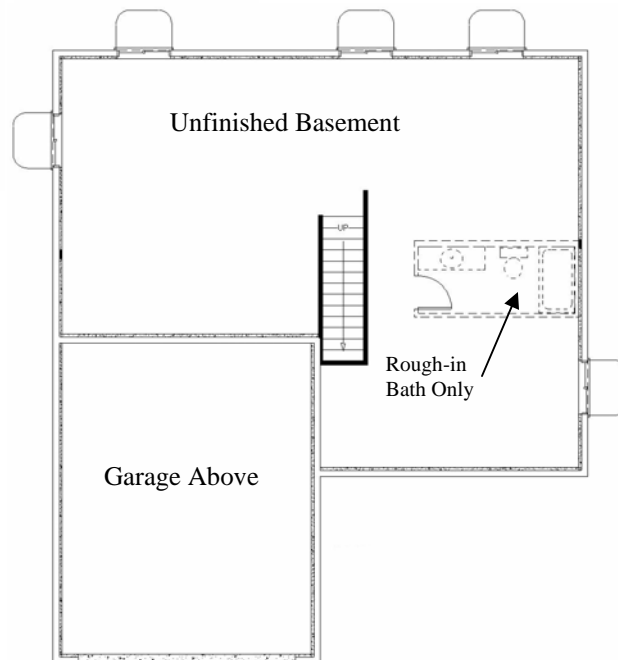
Unfinished Basement
